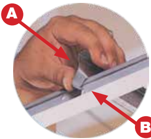
A Bend out tabs on ends of hangers
