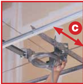
C Slide hangers with box or fixture housing attached along T Bar
