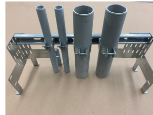
Multiple Conduit Sleeves on Strut with Strut Straps
