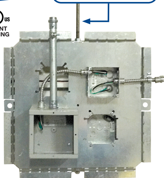
Vertical Installation Shown
